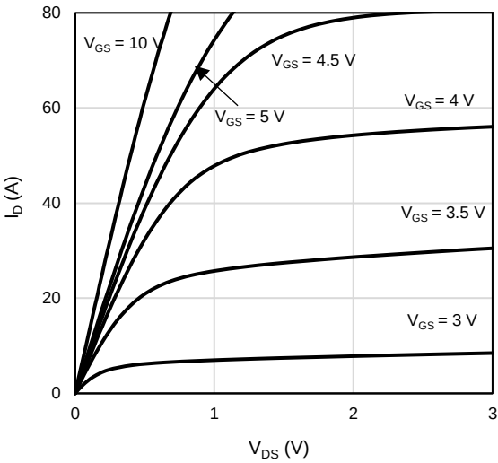
Figure 1: On-Region Characteristics
